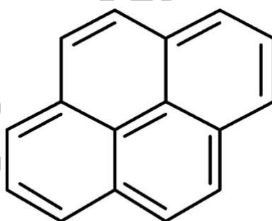
Figure 1. The structural formula of pyrene.
