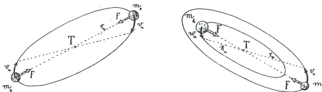
Figure 2. Mohorovičić's drawings in his 1934 paper of electrum (left) and nobelium (right).
